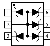
SC70-6L Pin Configuration
